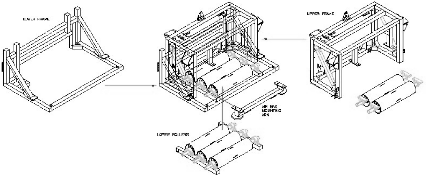
Exploded View
